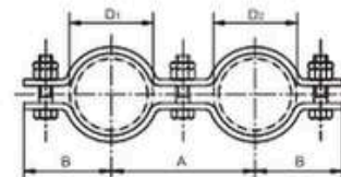
Multiple Pipe Clamps
